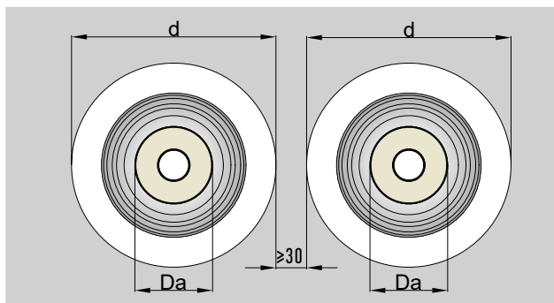
Abb. 38: Kernlochbohrung FibreFLEX/CaldoPEX single
